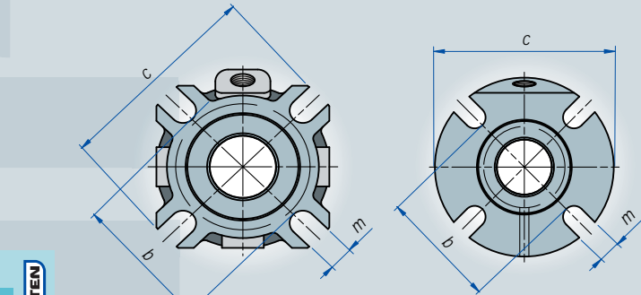
C3K e C3KC with shaft diameter ≤ 45 mm
